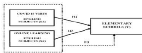
Fig 2. Hipotesis Model
